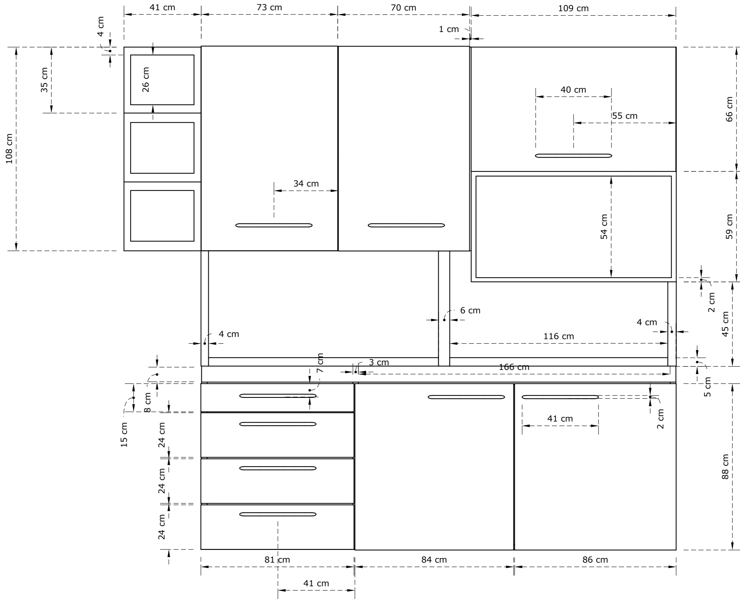
VISTA FRONTAL
